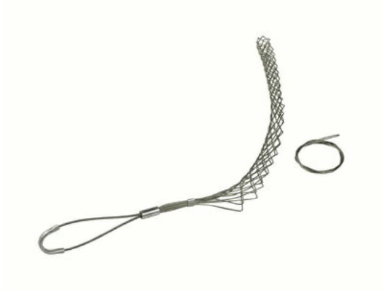
FS075OF: Standard Duty, Split Lace, Offset Eye, Cable Diameter 0.75 - 0.99 inches, Bale Length 4-in, Mesh Length 14-in
